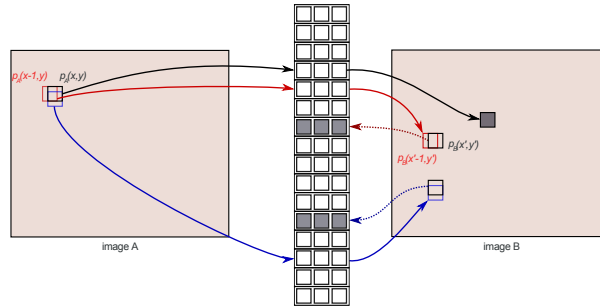
Fig. 4. Bin-Propagation in Spherical Hashing Scheme: If the spatial neighbor of p_A(x, y) (black patch), p_A(x - 1, y) (red), has a good match p_B(x' - 1, y') (red), the spatial neighbor of the match, p_B(x', y') (black) belongs to a bin in the Hash Table where all the patches are plausible candidates (shaded).
