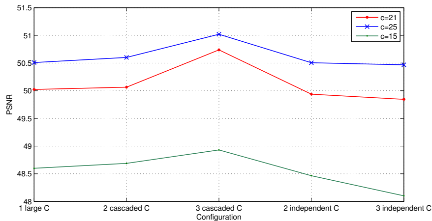
Fig. 7. Time-PSNR tradeoffs averaged on 225 reconstructions of independent images. The image size is 2Mp and the patch size is 3-by-3. 1 large C refers to a single spherical hashing system with large C , 2/3 independent C refers to configurations of independent hyperspheres systems with multiple tables, and 2/3 cascaded C refers to the proposed method. In the experiments, configurations for 2 and 3 stages with equal number of spheres as for 1 large C are: c_{15} = \{6, 9\}, \{4, 5, 6\} , c_{21} = \{8, 13\}, \{6, 7, 8\} and c_{25} = \{11, 14\}, \{7, 8, 10\} .
